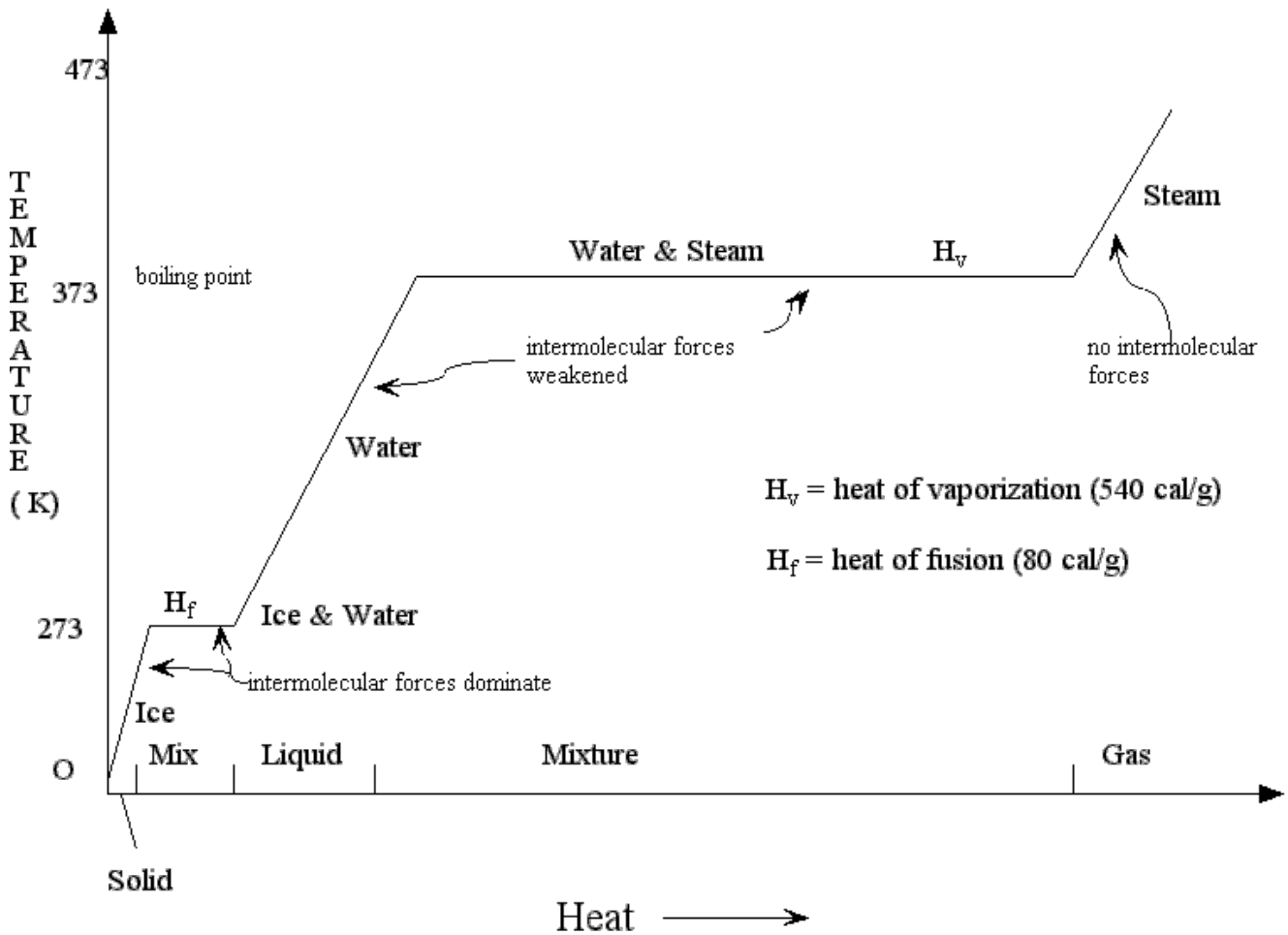
Phase Change Diagram for Water
